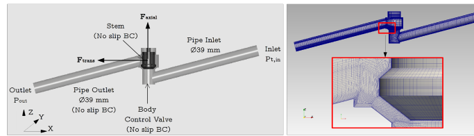
Figure 1: Computational domain and mesh
