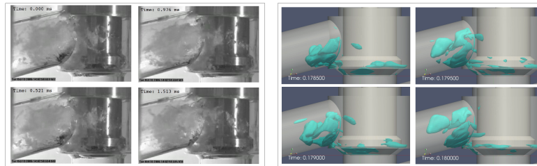
Figure 3: Experimental(Left) and numerical(Right) cavitation sequences, Lift 4mm
