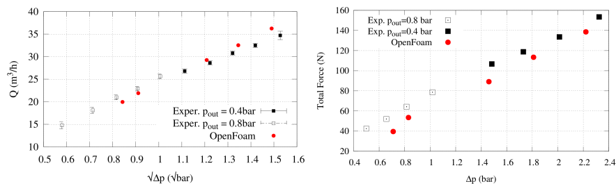
Figure 4: Flow rate vs \sqrt{\Delta P} (left) and force on the stem vs \Delta P (right), Lift 6 mm
