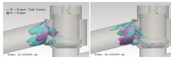
Figure 2: Pressure threshold turbulence correction
